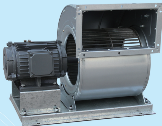
LKZ双进风电机直联通风机 LKZ Double-inlet Shaft-drive Centrifugal Fans
